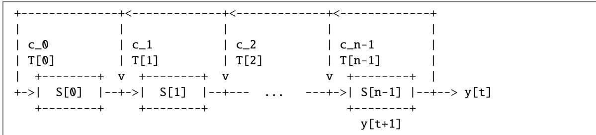
Listing 7: Galois LFSR Configuration
