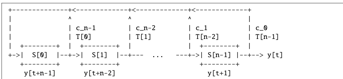
Listing 6: Fibonacci LFSR Configuration
